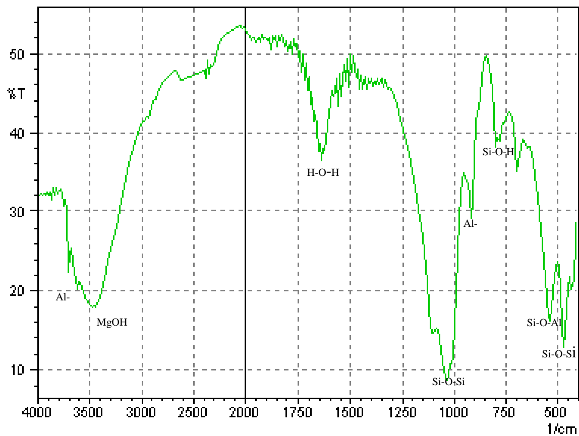
Figure 8.2: IR spectrum for Mutufu clay
