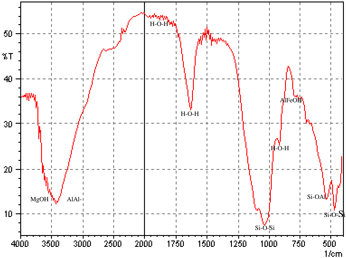
Figure 8.3: IR spectrum for Chelel clay
