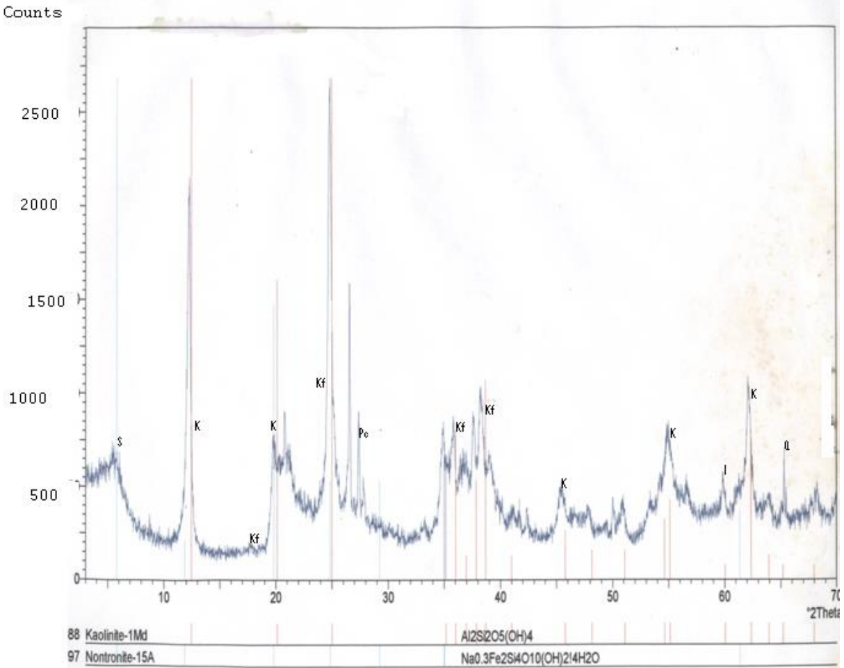
Figure 8.5b: XRD pattern of clay fraction settling after six days for clay from Chelel
